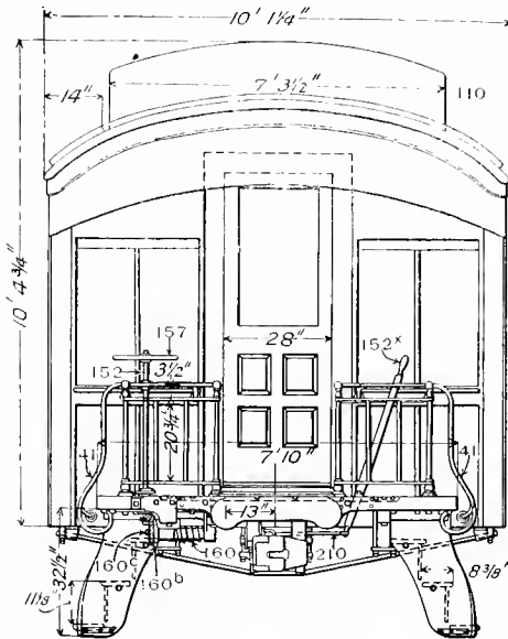
Fig 441. End Elevation.
